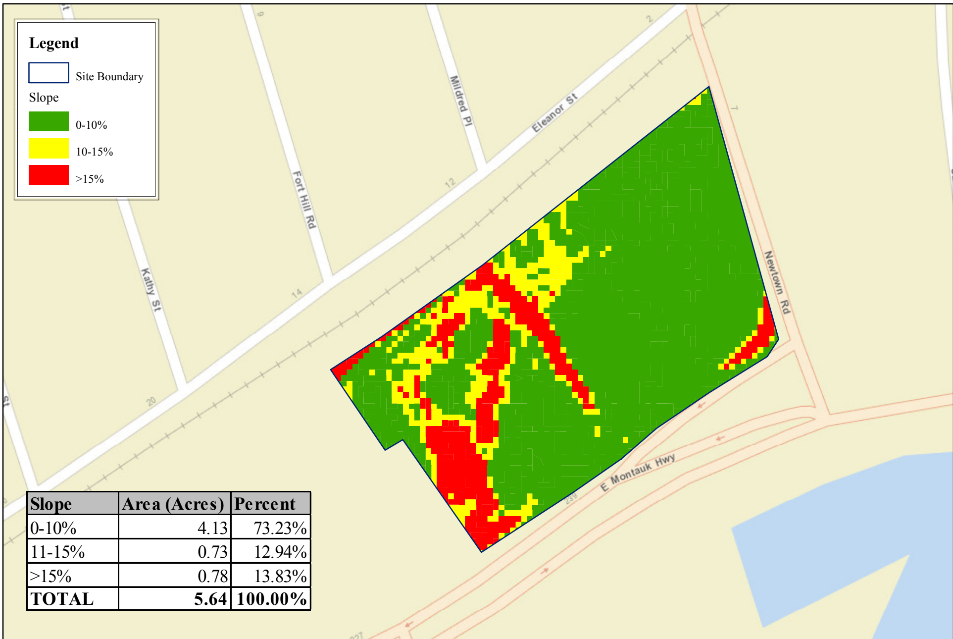
FIGURE 2-2a SLOPE ANALYSIS - CPI
